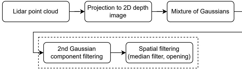
Figure 3.4. Steps of the proposed method for foreground-background separation in NRCS Lidar point clouds
