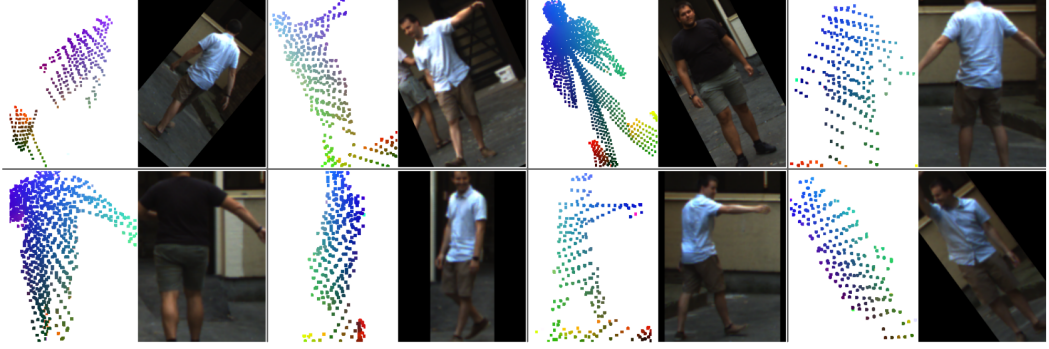
Figure 4.8. Example training batch of input data with the randomly applied augmentations (horizontal mirroring, scaling, rotation, half body transform). The camera images are shown for visual reference only.
