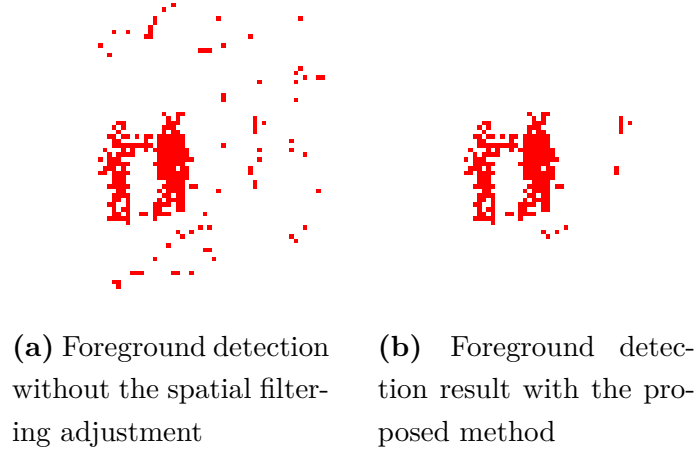
Figure 3.3. Foreground detection results in the central area of Figure 3.2a, displayed in range image representation.
