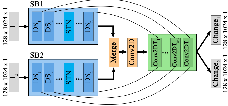
Figure 2.2. Proposed ChangeGAN architecture. Notations of components: SB1, SB2: Siamese branches, DS: downsampling, STN: spatial transformer network, Conv2DT: transposed 2D convolution
