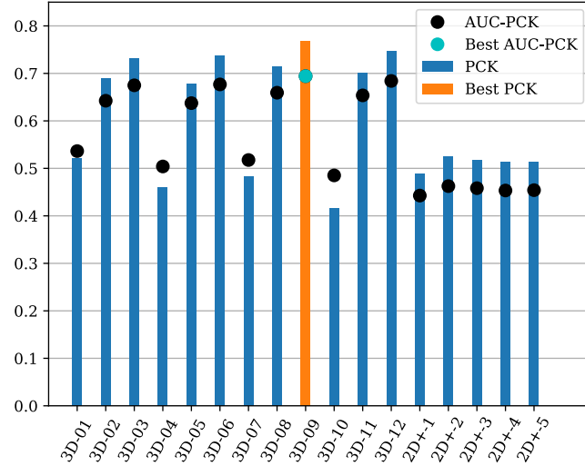
Figure A.1. PCK and AUC-PCK (both introduced in Section 4.4.1) values of the 3D predictions by LidPose-3D and LidPose-2D+ networks evaluated in 3D space with 3D metrics. The AUC-PCK was calculated on the [0, 0.5] meter interval, as shown in Figure 4.12
