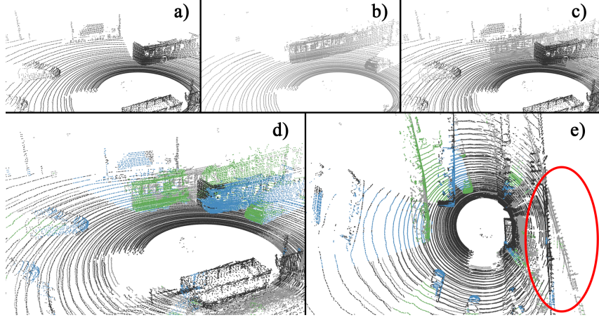
Figure 2.4. Changes detected by ChangeGAN for a coarsely registered point cloud pair. (a) and (b) show the two input point clouds, (c) displays the coarsely registered input point clouds in a common coordinate system. (d),(e) present the change detection results: blue and green colored points represent the objects marked as changes in the first- and second point cloud, respectively. The red ellipse draws attention to the global alignment difference between the two coarsely registered point clouds.
