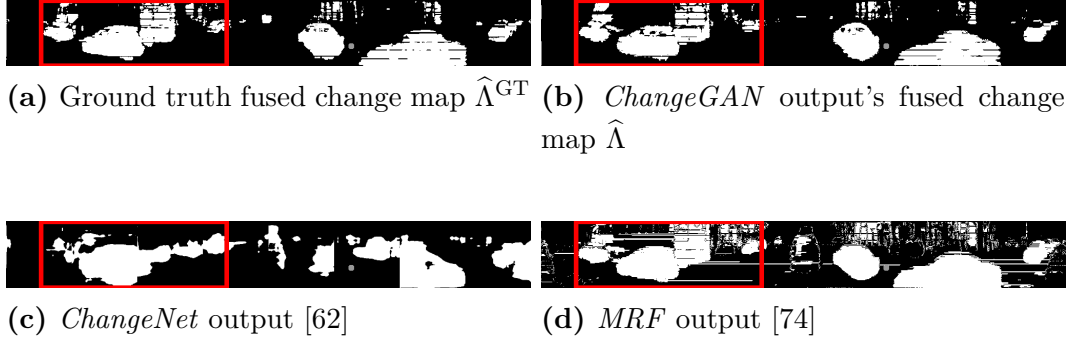
Figure 2.5. Predicted change masks by the different methods on input data, shown in Figure 2.1. Red rectangles: region displayed in 3D in Figure 2.8.
