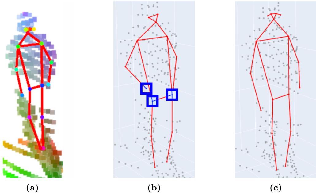
Figure 4.3. Predicted human poses of the LidPose variants, overlaid on the input data.
