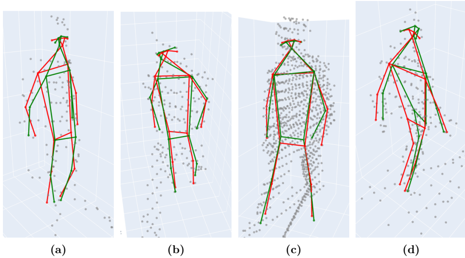
Figure 4.14. LidPose3D predicted skeletons using the 3D-09 configuration. Red skeleton: 3D prediction. Green skeleton: GT. Gray points: NRCS Lidar points.
