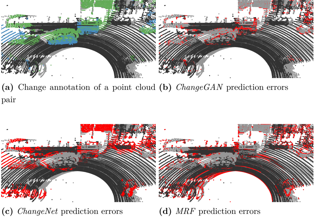
Figure 2.9. Prediction errors samples of the ChangeGAN and the reference methods
