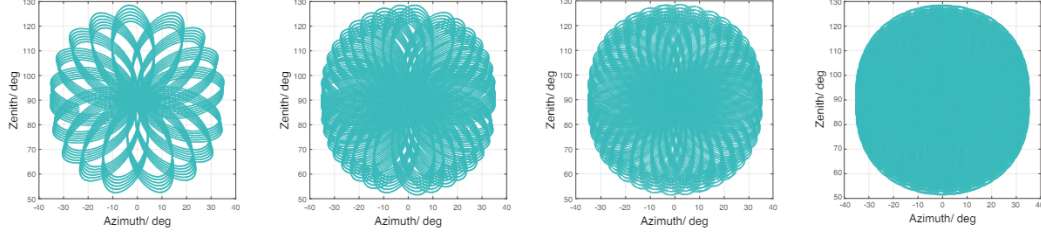
Figure 1.6. Typical point cloud pattern inside the FoV of the Livox Avia Lidar sensor after (from left to right) 0.1 seconds, 0.5 seconds, 1 second, 3 seconds. Source: [56]
