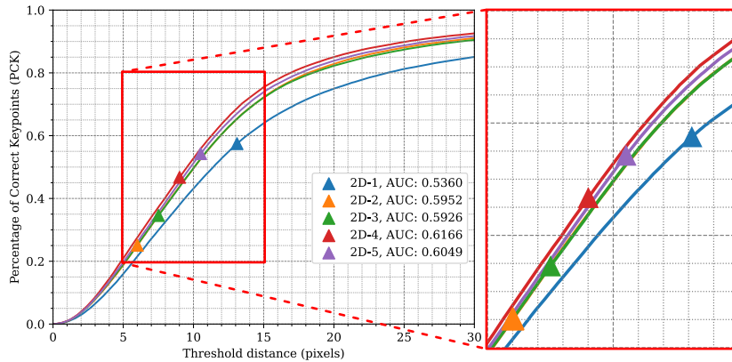
Figure 4.9. LidPose-2D : Percentage of Correct Keypoints for the different 2D networks with different joint-correspondence threshold acceptance values. Model 2D-4 , which has been trained on 3D coordinates + Lidar intensity, has the best PCK curve.
