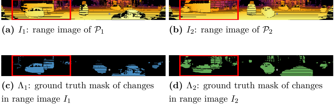
Figure 2.1. Input data representation. (a), (b): range images I_1, I_2 from a pair of coarsely registered point clouds \mathcal{P}_1 and \mathcal{P}_2 . (c), (d): binary ground truth change masks \Lambda_1, \Lambda_2 for the range images I_1 and I_2 , respectively. The red rectangle marks the region displayed in 3D in Figure 2.8.
