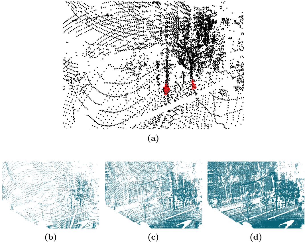
Figure 3.6. Evolution of the high-resolution background model in the City Center dataset
