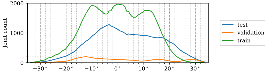
Figure 4.5. Distribution of the joints recorded in the LidPose dataset, based on the local emergence angle of the Lidar sensor
