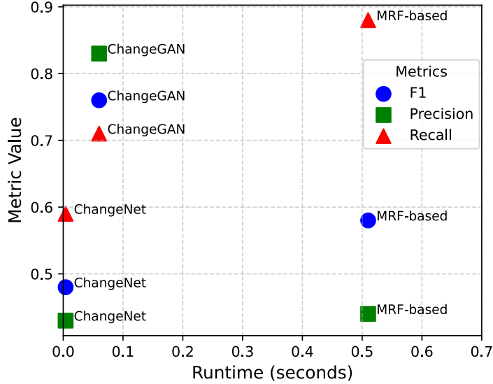
Figure 2.6. Execution time and performance of the proposed ChangeGAN method against the ChangeNet [62] and the MRF -based reference approach [74]
