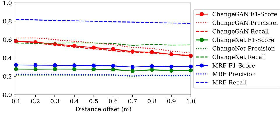
Figure 2.10. Translation dependency of the compared methods’ performance (F1-score, Precision, Recall)
