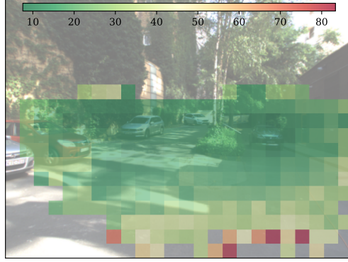
Figure 4.10. 2D Average Distance Error of the selected 2D-4 model, overlaid on a sample camera image.
