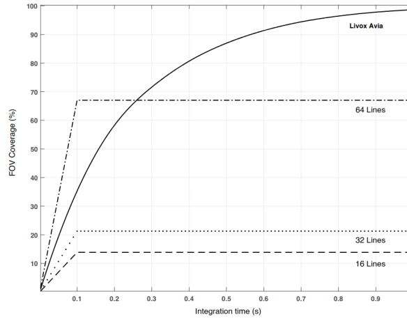
Figure 1.5. Change in FOV coverage over time for the Livox Avia compared to rotating multi-beam sensors with traditional scanning. Source: [56]
