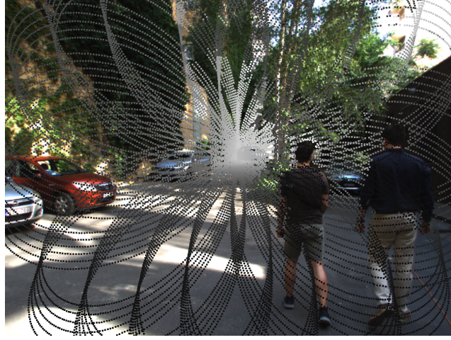
Figure 1.4. NRCS Lidar point cloud with 100 ms integration time represented as a 2D range image overlaid on a sample camera image. The point cloud is colored by the distance: the lighter the point's color, the greater its distance.
