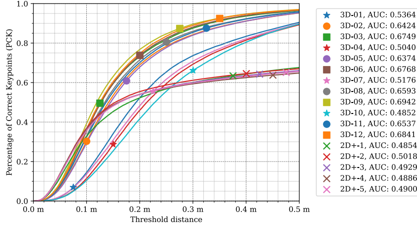
Figure 4.12. LidPose-3D : Percentage of Correct Keypoints in the 3D space for the different 3D (and 2D+) networks with different joint-correspondence threshold distance acceptance values. Model 3D-9 , which has been trained on 3D coordinates + Lidar intensity with SSIM-based depth loss, has the best PCK curve.
