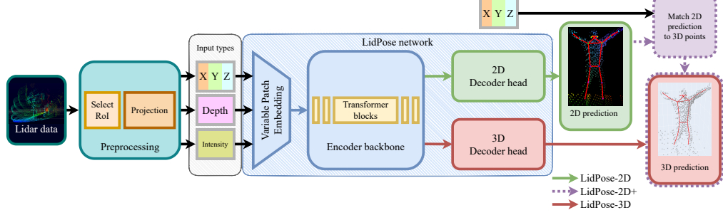
Figure 4.2. LidPose end-to-end solution:
