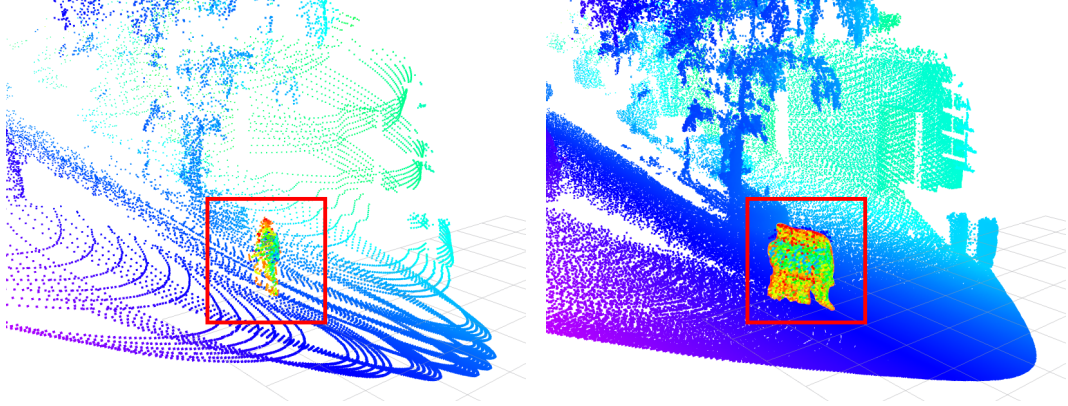
(a) NRCS Lidar point cloud with 100 ms integration time (b) NRCS Lidar point cloud with 1000 ms integration time
