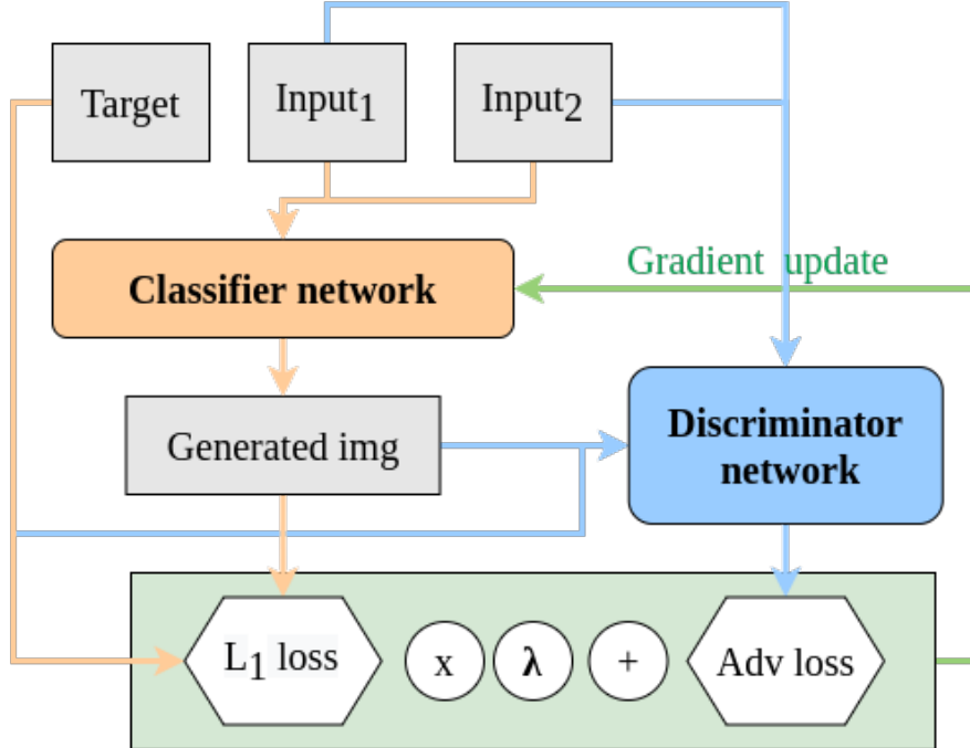
Figure 2.3. Proposed adversarial training strategy of the ChangeGAN architecture.
