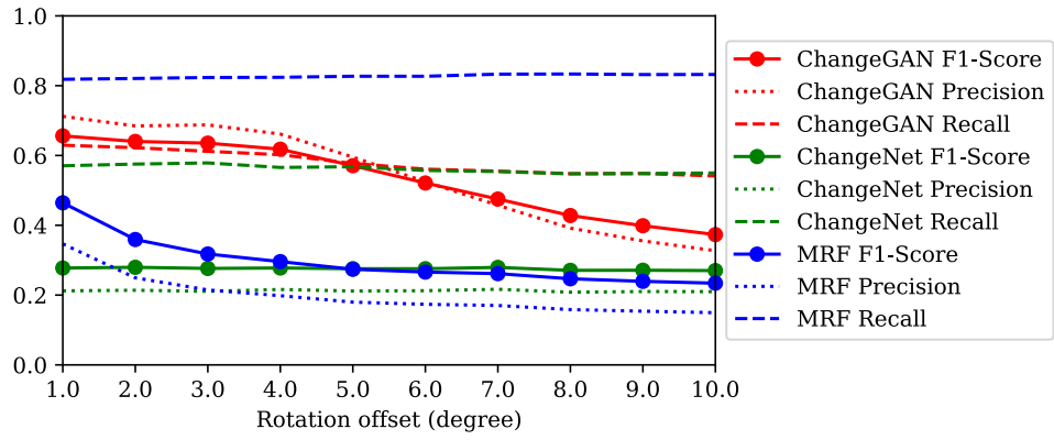
Figure 2.11. Translation rotation dependency of the compared methods' performance (F1-score, Precision, Recall)
