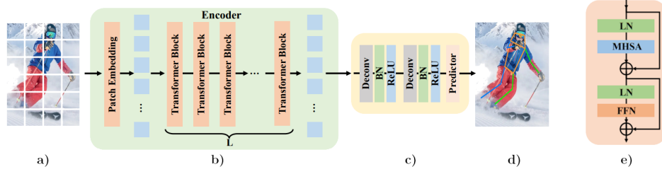
Figure 4.1. The structure of the ViTPose method [33].
