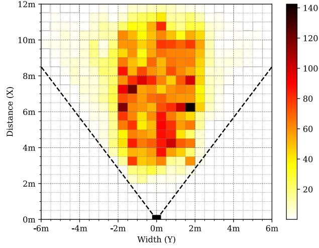
Figure 4.6. Distribution of joint positions in the LidPose dataset, displayed on the ground plane (X, Y)_{3D} from the bird's-eye view.
