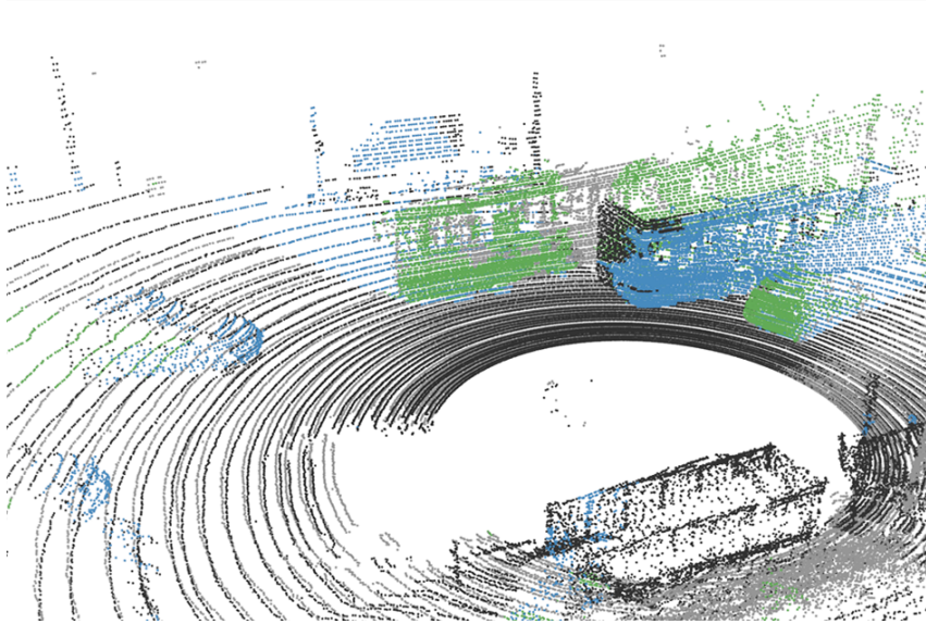
Figure 2.7. Changes detected by ChangeGAN for a coarsely registered point cloud pair. Blue and green points represent the changes in the first and second point clouds.
