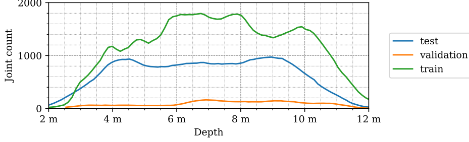
Figure 4.4. Distribution of the joints in the LidPose dataset, based on the depth coordinate ( X ) of the 3D joints.
