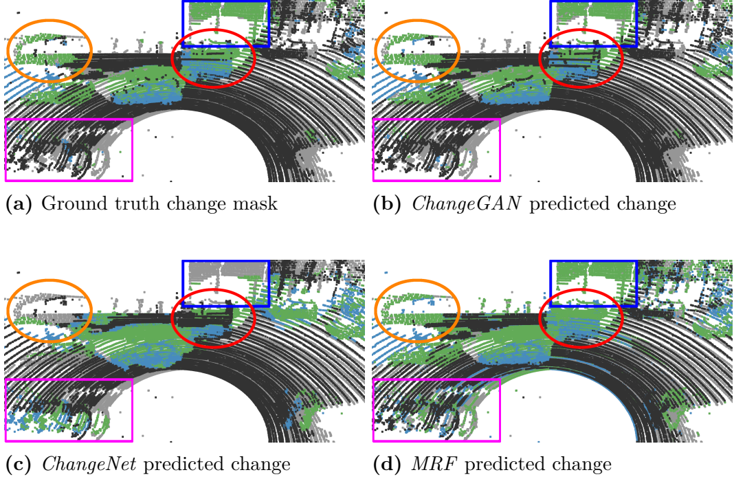
Figure 2.8. Comparative results of the ground truth and the predicted changes by ChangeGAN and the reference techniques. Green and blue points mark changed regions in \mathcal{P}_1 and \mathcal{P}_2 respectively. Orange and red ellipses mark the detected front and back part of a bus traveling in the upper lane, meanwhile occluded by other cars. The blue square shows a building facade segment, which was occluded in \mathcal{P}_2 . The magenta boxes highlight false positive changes of the reference methods confused by inaccurate registration.
