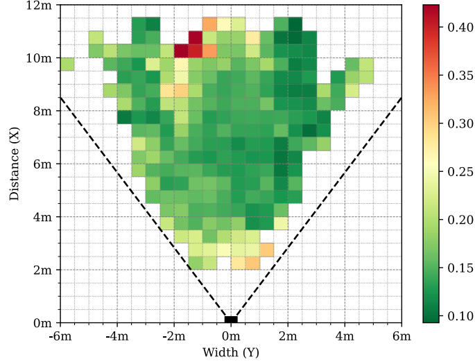
Figure 4.13. Distribution of Average Distance Error of the predicted joints in bird’s eye view, using the selected 3D-09 model. Only cells with more than 24 annotated joints are shown.
